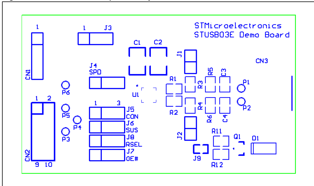
Figure 3. Demo board components layout
