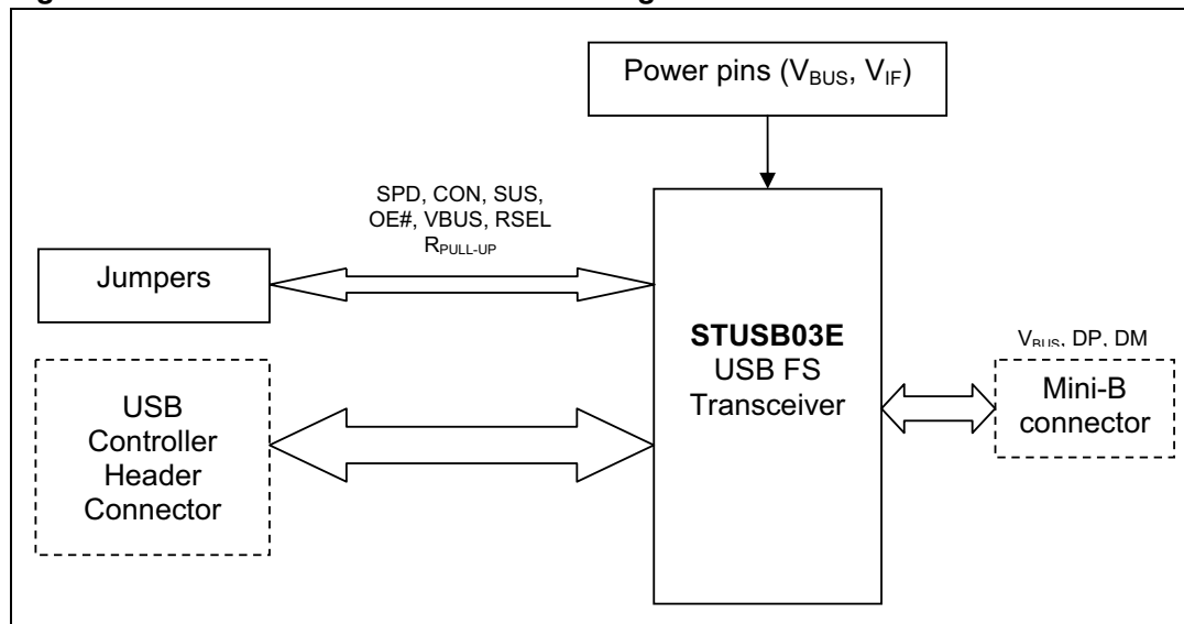
Figure 1. STUSB03E demo board block diagram
